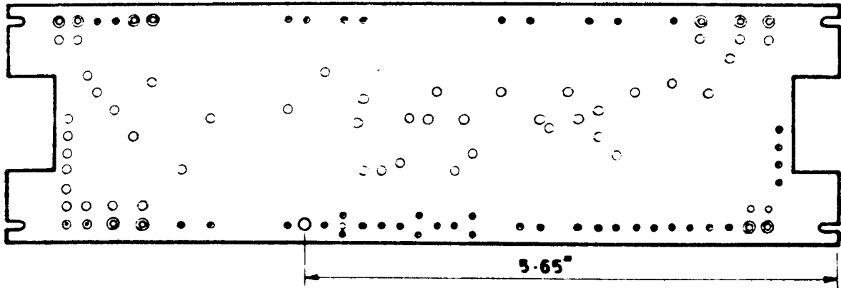
Figure 3-5 Location of terminal LS10
