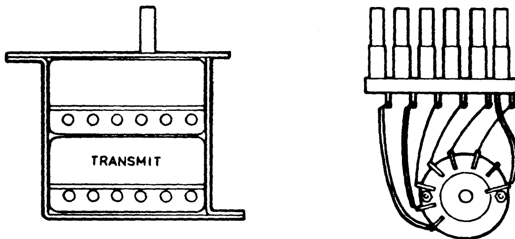
Figure 3-13 Transmit Channel Crystal Assy Connections
