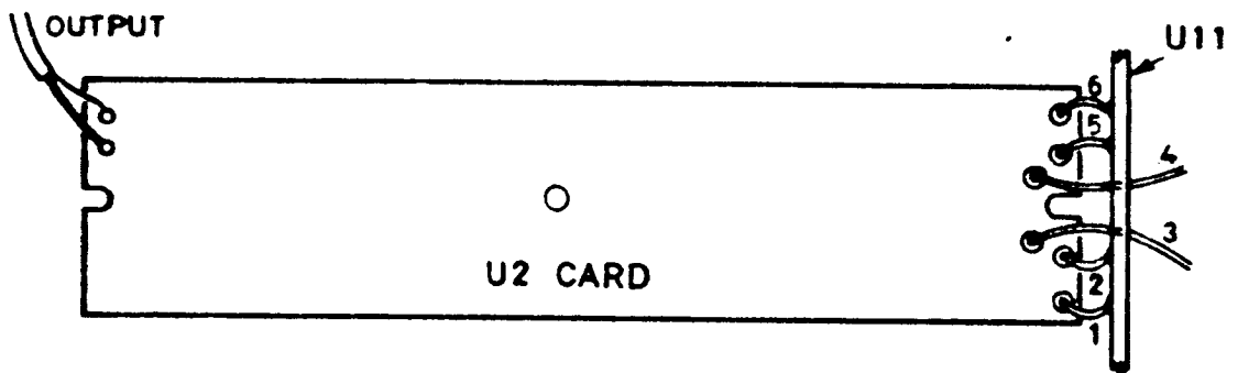
Figure 3-14 Exciter Card U2 Connections
